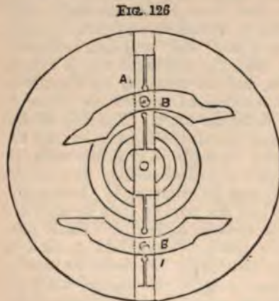
Dunning's turn-table.
